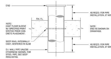
FLOOR PIPE "A" DETAIL NO SCALE
