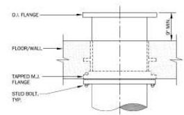
FLOOR PIPE SLEEVE DETAIL NO SCALE
