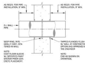
DUCTILE IRON WALL PIPE DETAIL NO SCALE
