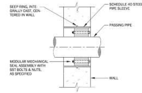
WALL PENETRATION SEAL DETAIL NO SCALE
