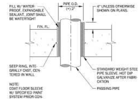
FLOOR PIPE SLEEVE DETAIL NO SCALE
