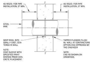
CONCRETE WALL PIPE PENETRATION DETAIL NO SCALE
