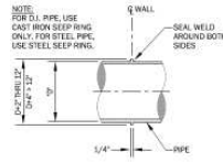
SLEEP RING DETAIL NO SCALE
