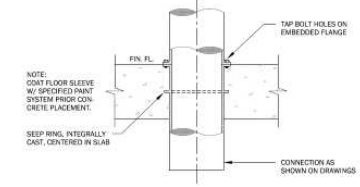
FLOOR PIPE "B" DETAIL NO SCALE
