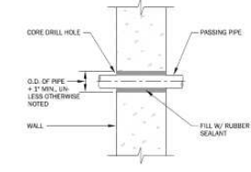
WALL PIPE PENETRATION DETAIL NO SCALE
