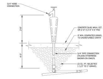
NON-FREEZE POST HYDRANT DETAIL NO SCALE
