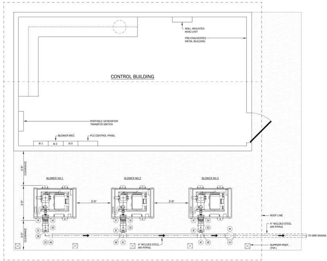
PLAN VIEW
